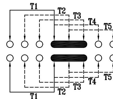
SCHEMATIC (SHORTING)
